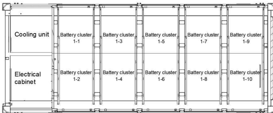
Figure 2.4.1-1 Internal layout of a Single Container
