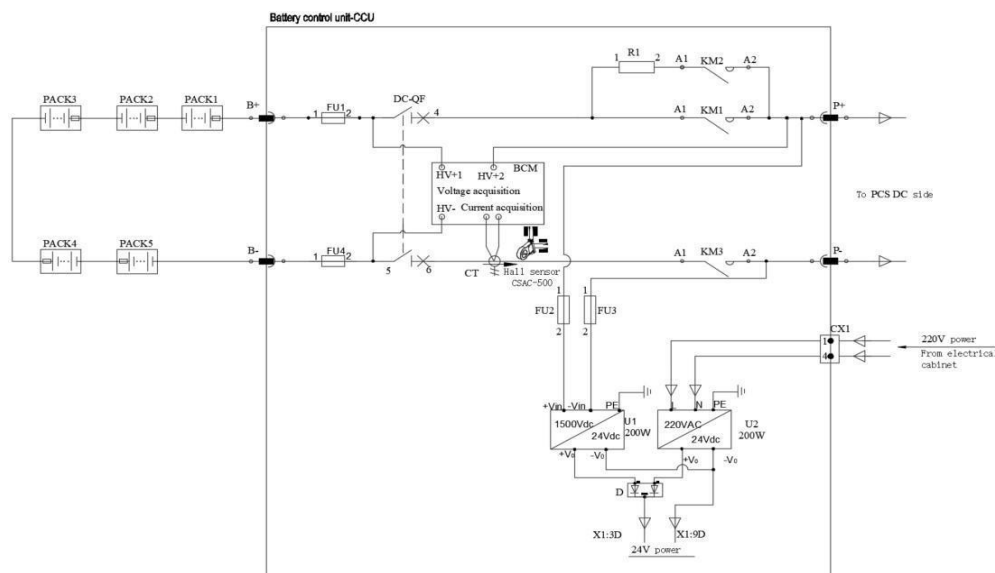
Figure 3.2.2-1 CCB primary diagram
