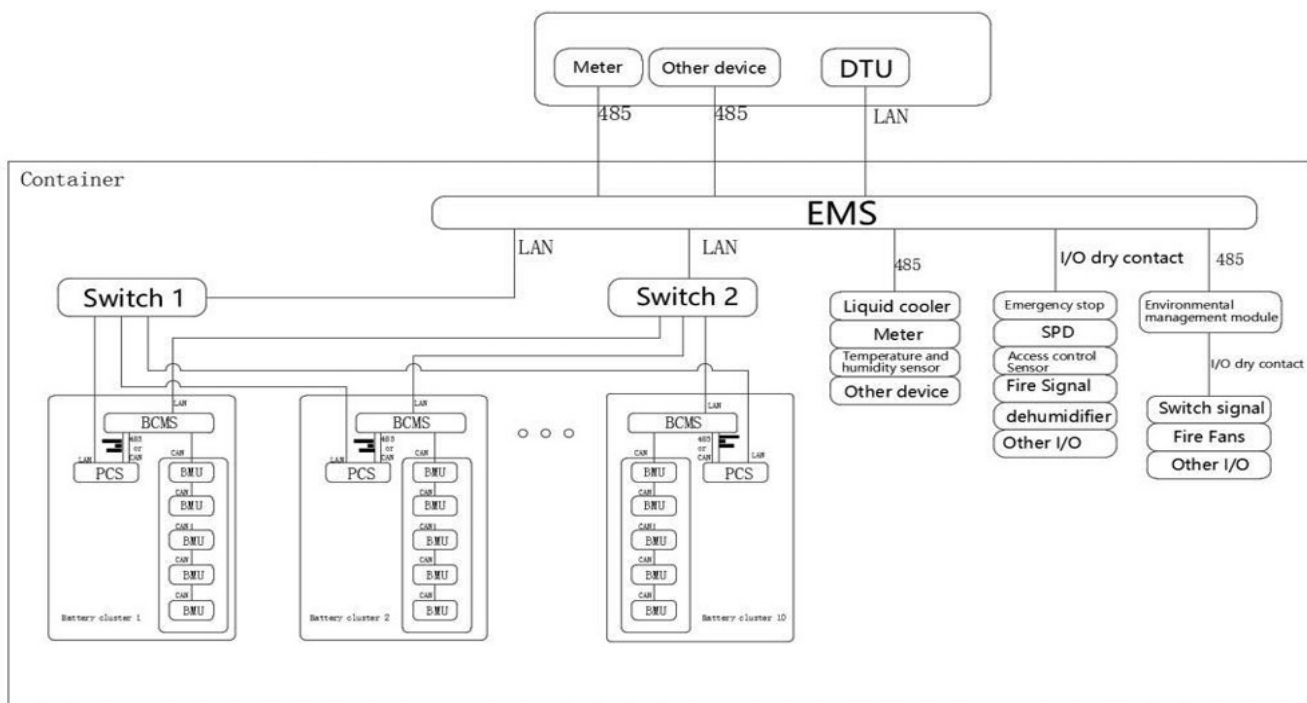
Figure 3.6-1 Communications topology
