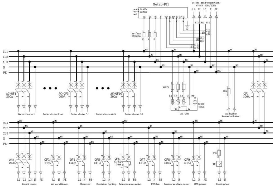
Figure 2.3-1 Primary Electrical Schematic
