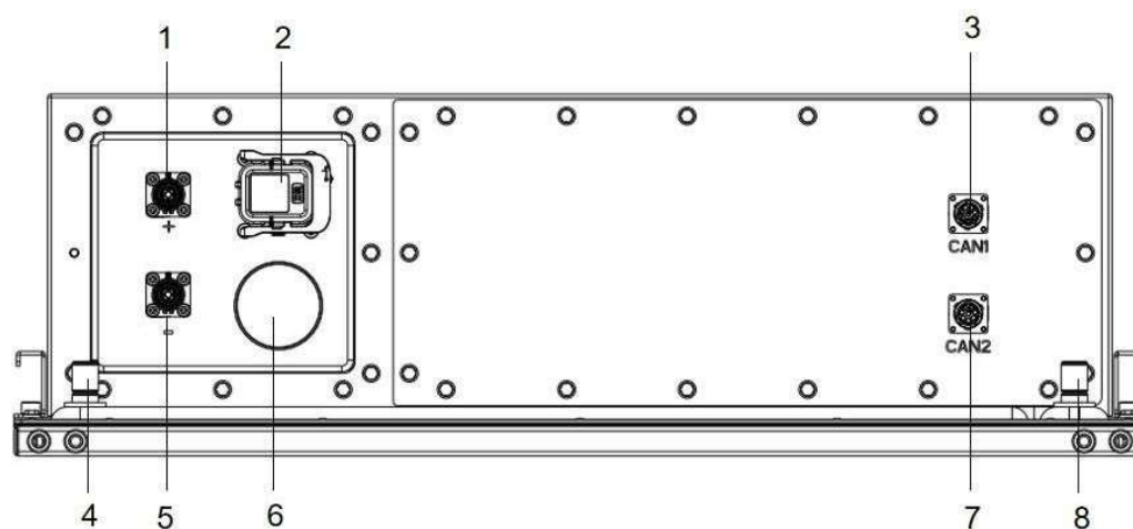
Figure 3.1-1 Battery Module
