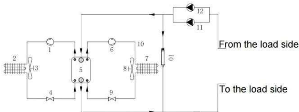
Figure 3.3.4-1 Chiller schematic diagram
